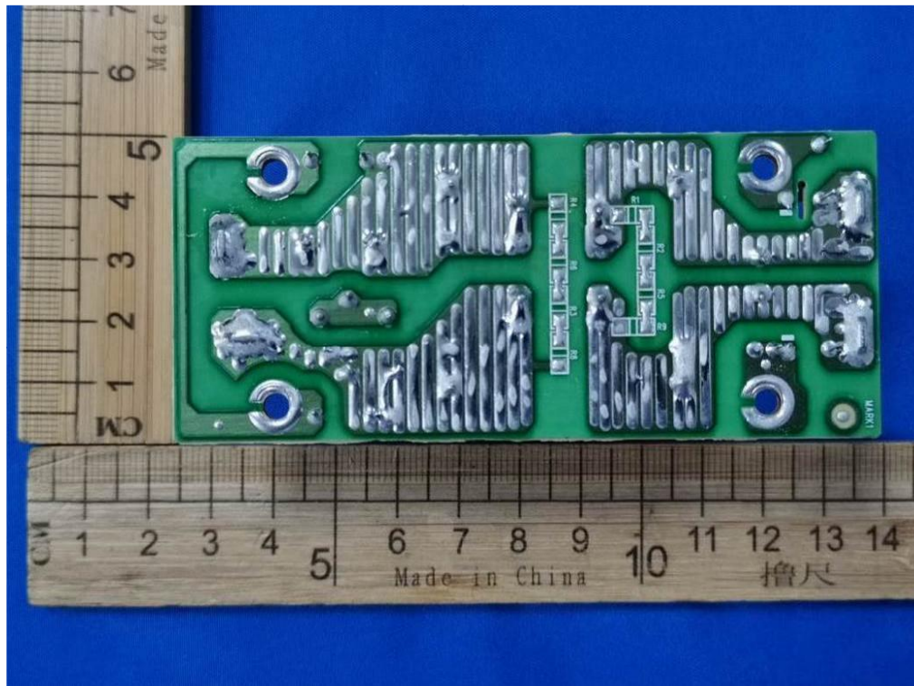
Figure 20: Filter of PCB(1.5K)
