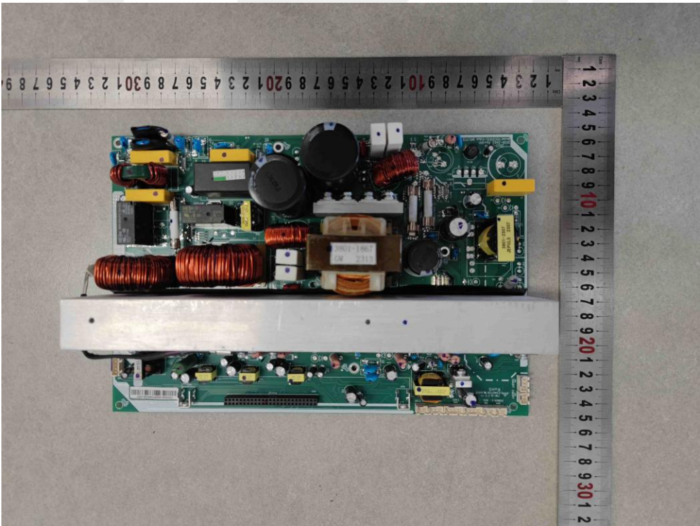
Figure 27: PCB view(2K)
