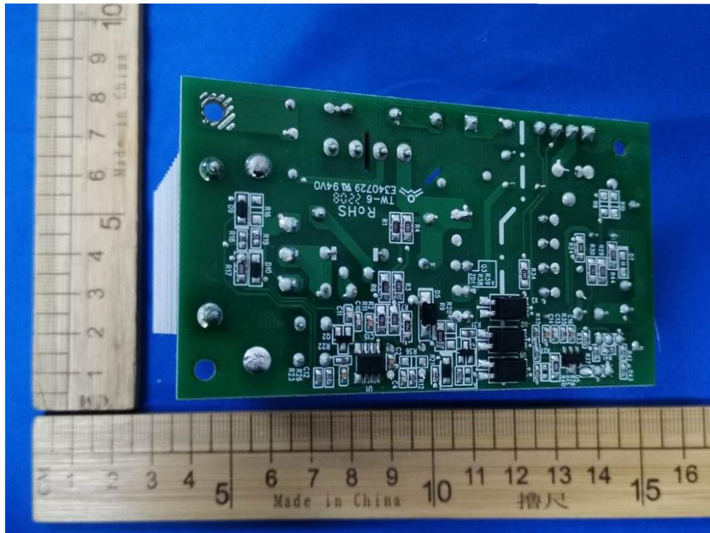
Figure 9: Trace side of PCB(3K)
