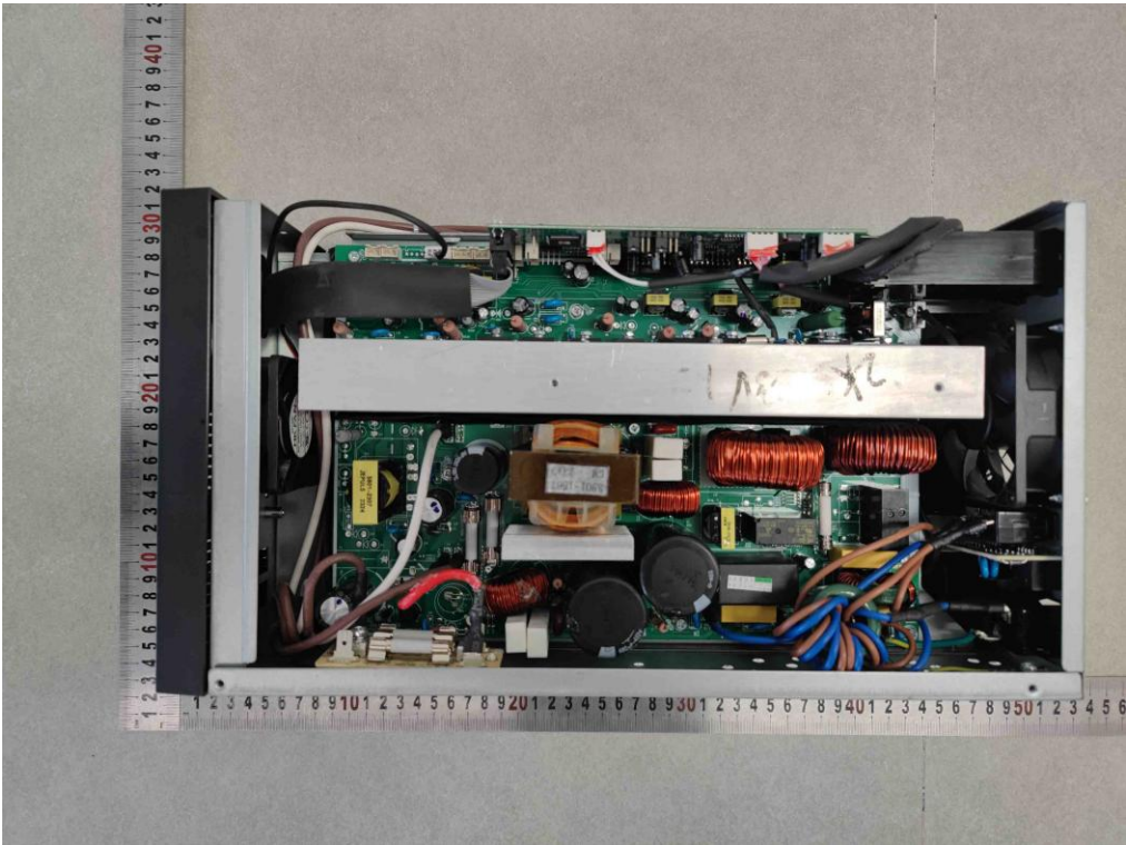
Figure 26: Internal view(2K)
