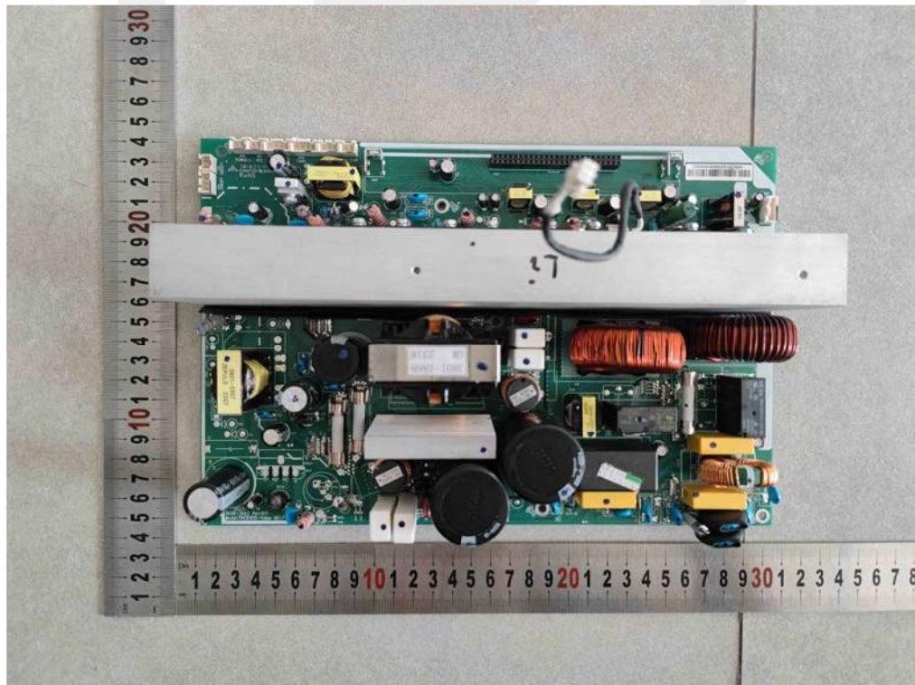
Figure 17: Component side of PCB(1.5K)
