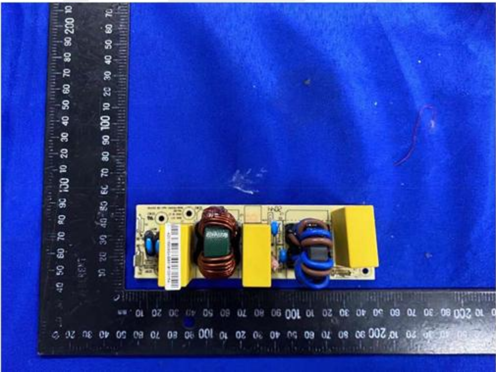
Figure 12: Component side of PCB(3K)
