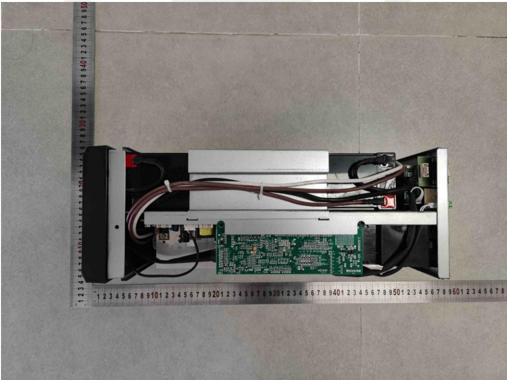
Figure 25: Internal view(2K)
