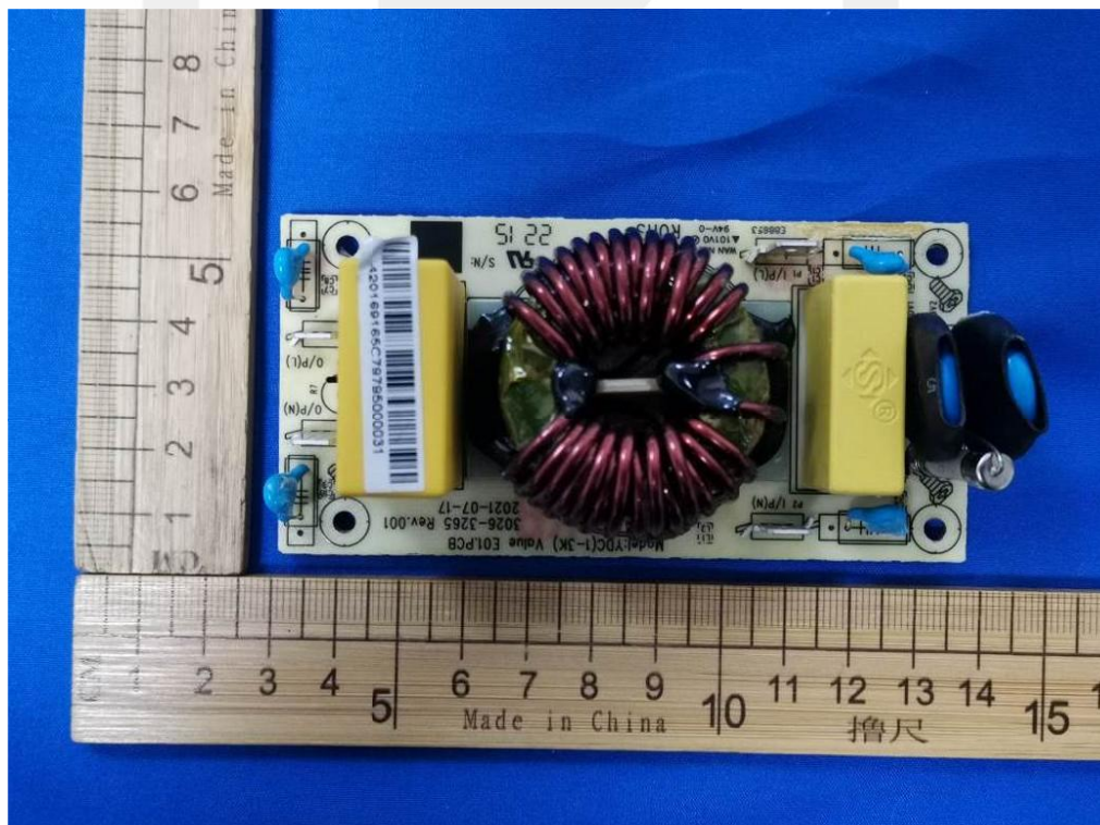
Figure 10: Filter of PCB(3K)
