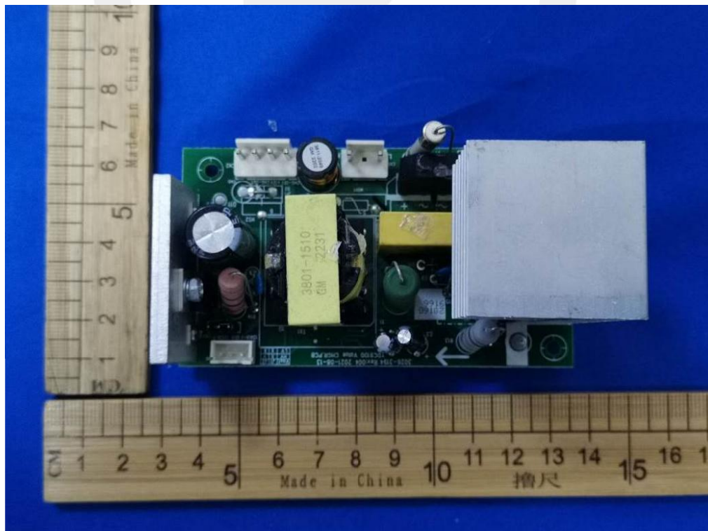
Figure 8: Trace side of PCB(3K)
