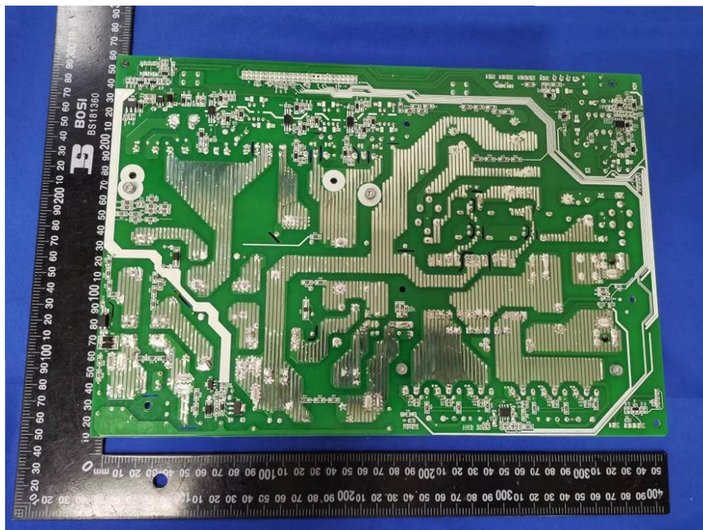
Figure 5: Trace side of PCB(3K)
