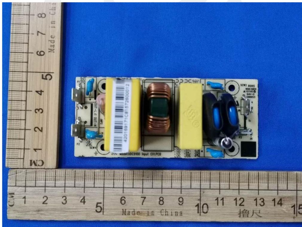
Figure 19: Filter of PCB(1.5K)
