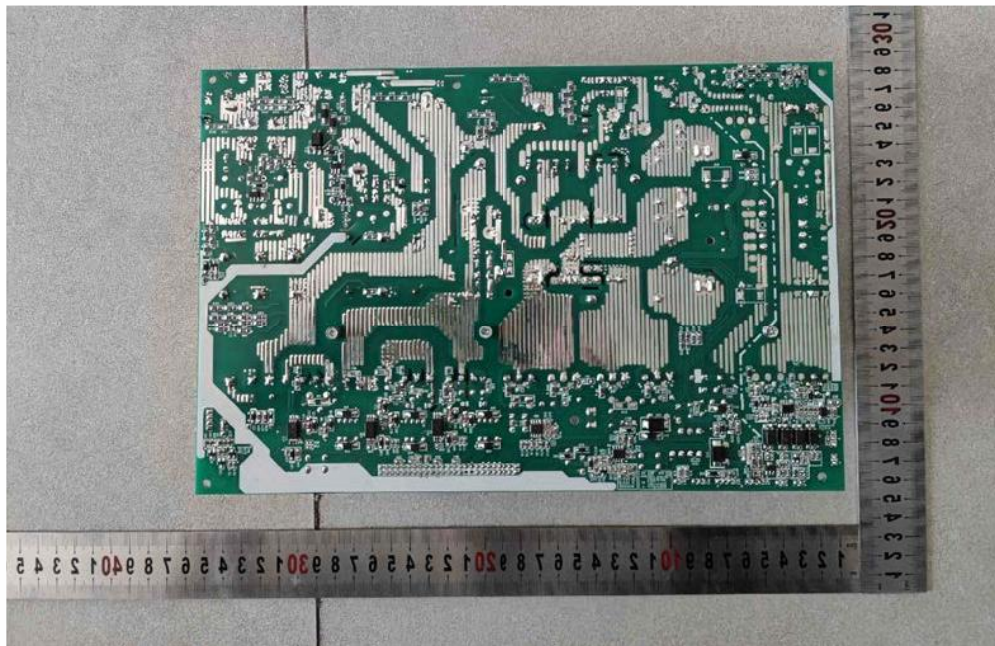
Figure 18: Component side of PCB(1.5K)
