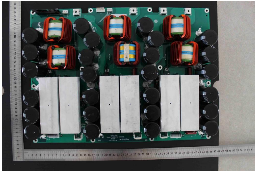
PCB view
