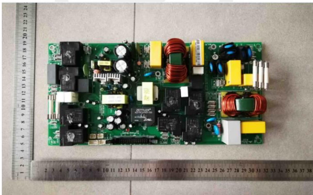
Figure 6: PCB view
