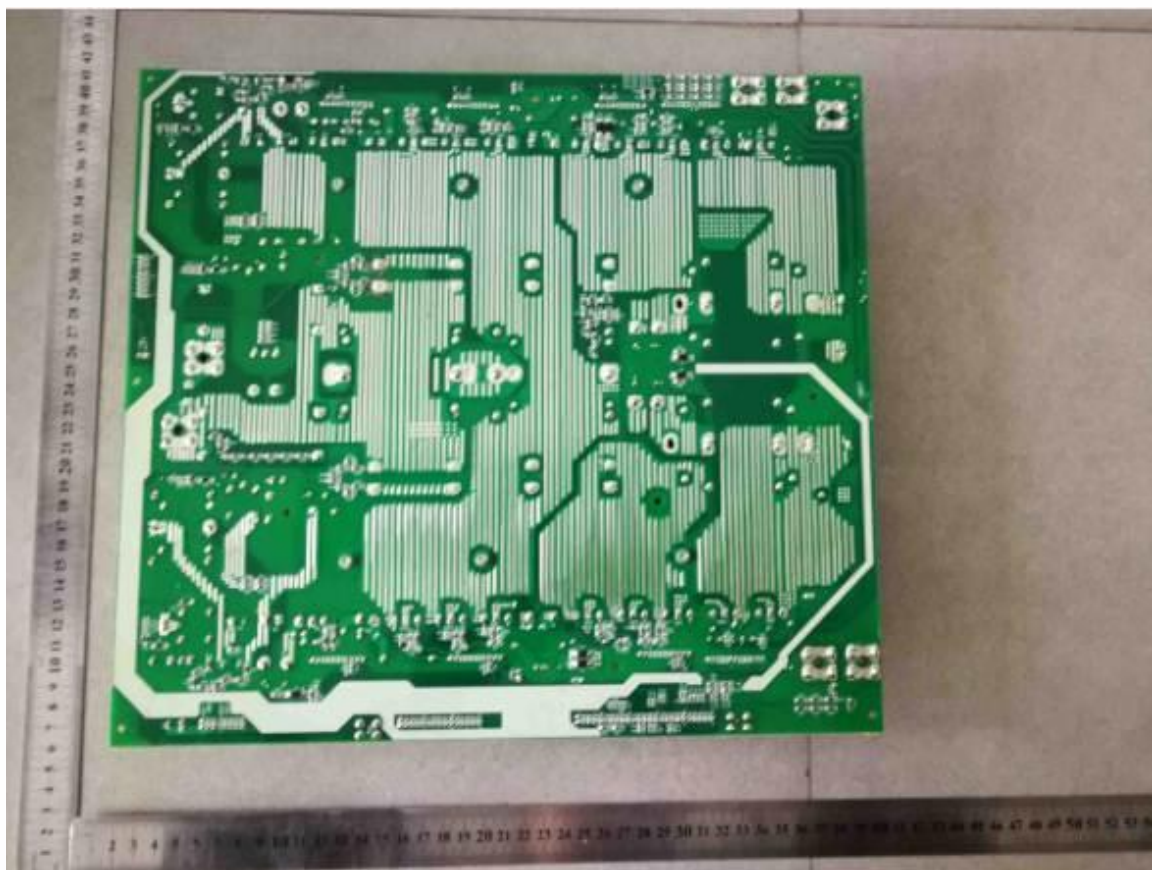
Figure 5: PCB view
