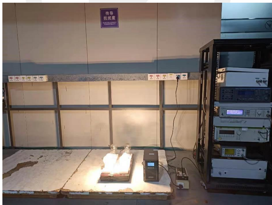
17.8.Photo of Injected Currents Susceptibility Test
