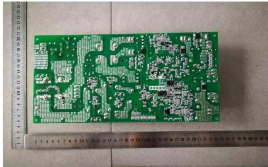
Figure 7: PCB view
