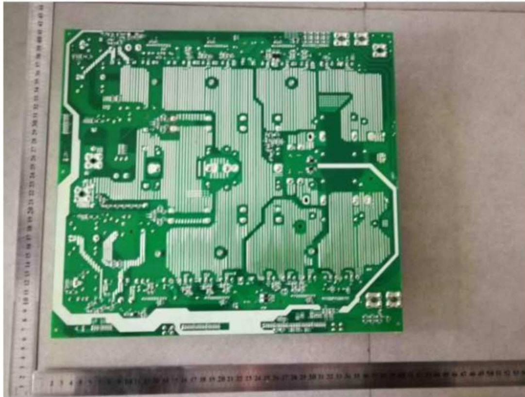
Figure 5: PCB view
