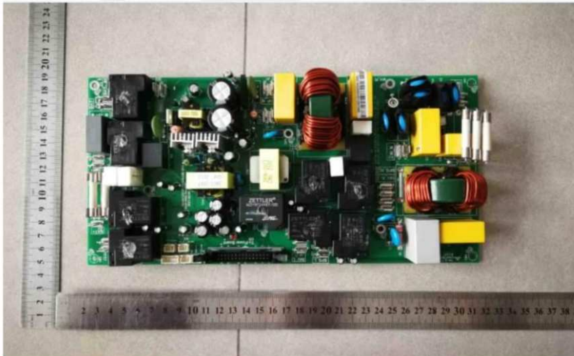
Figure 6: PCB view
