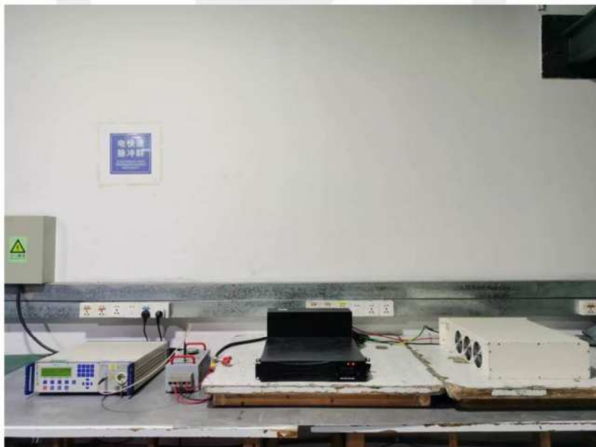
17.6.Photo of Electrical Fast Transient / Burst Test
